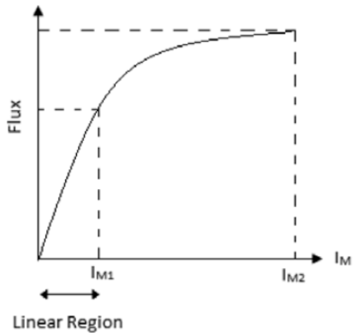
Figure 1 - Magnetization curve of current transformer
